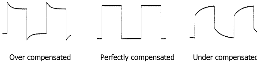
Figure 1-12 Probe Compensation
