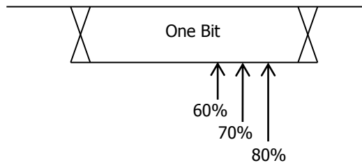
Figure 12-10 Sample Position
