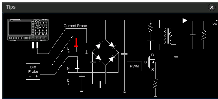
Figure 8-1 Connection Diagram of Power Quality Analysis
