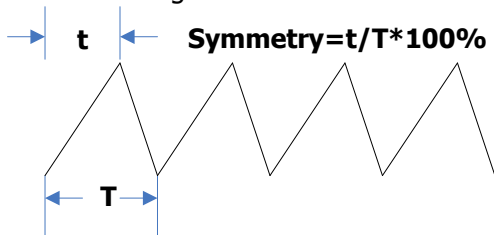
Figure 18-1 Symmetry Definition
