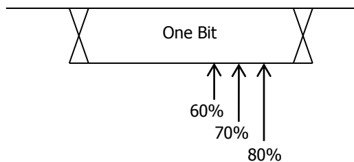
Figure 12-12 Sample Position
